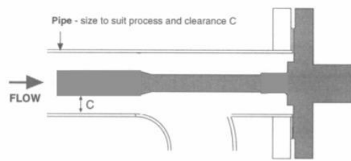
PIPE ELBOW MOUNTING - OPTIMUM INSTALLATION Minimum pipe clearance C = 8mm
